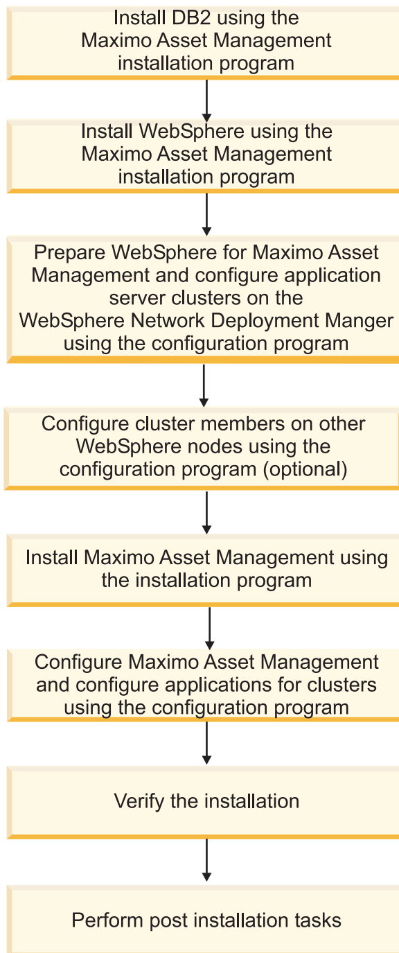
Figure 14. Deploying Maximo Asset Management using automatic middleware configuration
