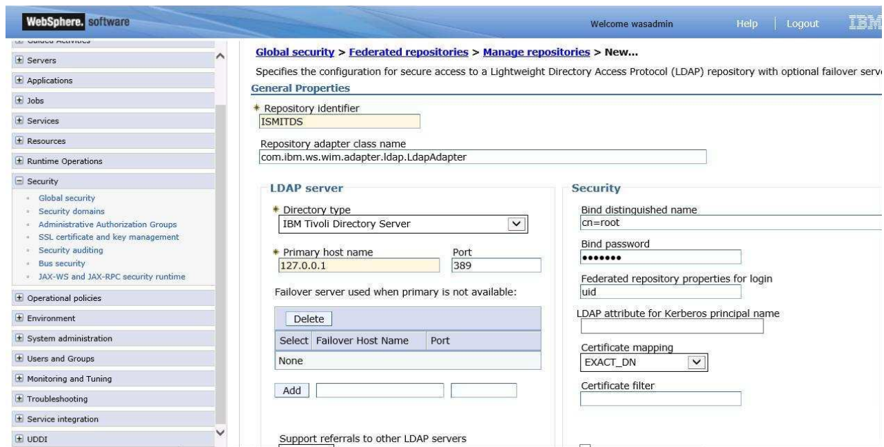
Figure 13. New Repository
